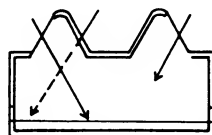
(c) opposed inclined surfaces (note corner illumination)
